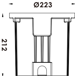
Mounting sleeve
