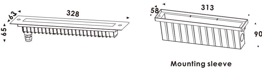
Mounting sleeve
