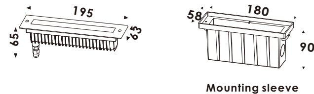
Mounting sleeve
